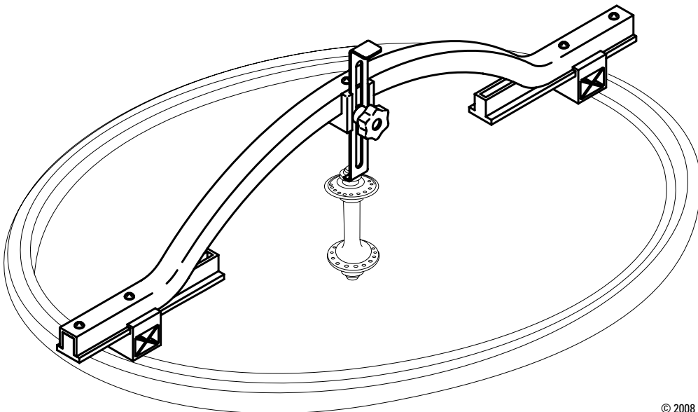
WAG-4 Wheel Alignment Gauge
